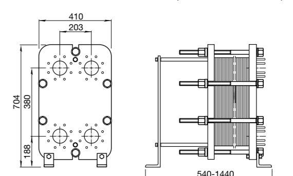
FD Dimensions (measurements in mm)
