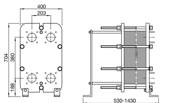
FG Dimensions (measurements in mm)
