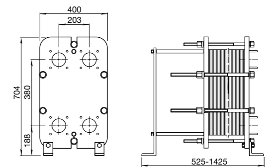
FM Dimensions (measurements in mm)
